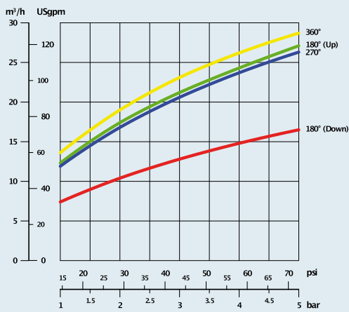
Pressure/Flow (Clip)
