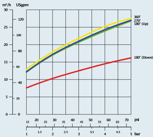
Pressure/Flow (BSP)
